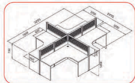
MT-WS014C 3255(W) x 2455(D) x 1200(H) mm.
