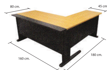
MAJOR(L,R) W160,180 x D80,45 x H75 cm.
